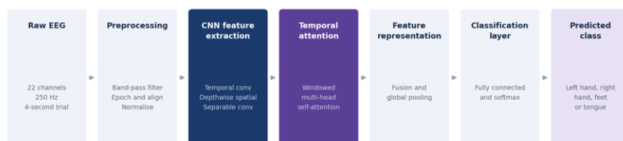
Figure 7.1 — System architecture. The two shaded stages are the learned components that together form the proposed model; the remaining stages are fixed signal processing and output layers.
